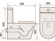
● WC-6014 Washdown Close Coupled Toilet
