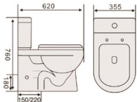
● WC-8011 Washdown Close Coupled Toilet
