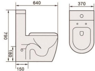
● WC-1039 Washdown One-piece Toilet
