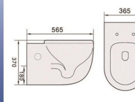
● WC-6019 Washdown Wall-hung Pan
