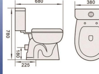
● WC-3887 Washdown Close Coupled Toilet
