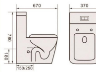
● WC-6018 Washdown Care Toilet Suits
