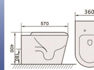
● WC-6015 Washdown Back-to-wall Pan
