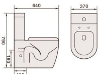
● WC-6009 Washdown Close Coupled Toilet
