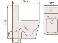
● WC-6002 Washdown Close Coupled Toilet
