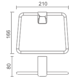
29201422 Towel ring Material: Zinc alloy Finish: Black Number: 0022800
