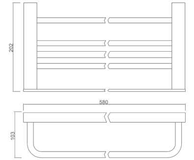
15901301 Towel rack Material: SUS304 Finish: Brushed Number: 0053500
