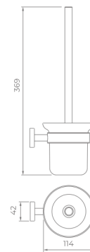
23601109 Toilet brush holder Material: Brass Finish: Black Number: 0021700
