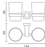
22402100 Double cups holder Material: Brass Finish: Chrome Number: 0022800
