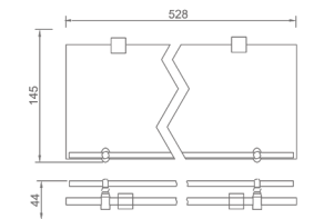
47503109 Glass shelf Material: Brass Finish: Black Number: 0019500
