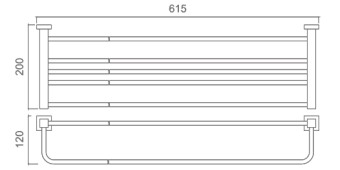
22902100 Towel rack Material: Brass Finish: Chrome Number: 0087500
