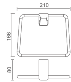
29201400 Towel ring Material: Zinc alloy Finish: Chrome Number: 0019000
