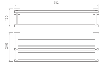
23901100 Towel rack Material: Brass Finish: Chrome Number: 0089500
