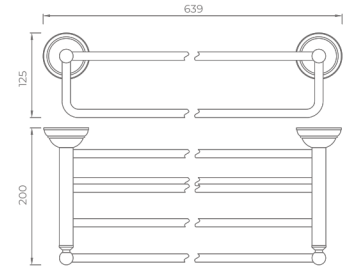
27901100 Towel rack Material: Brass Finish: Chrome Number: 0069800
