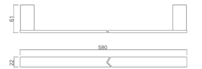
1510 13 2 3 Single towel bar Material: SUS304 Finish: Gun gray Number: 0035780
