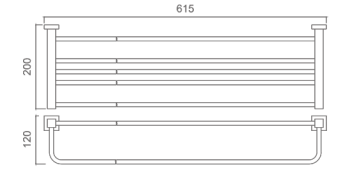
22902122 Towel rack Material: Brass Finish: Black Number: 0102000
