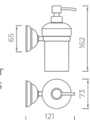
27503100 Soap dispenser holder Material: Brass Finish: Chrome Number: 0026250
