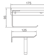
10812301 Tissue holder Material: SUS304 Finish: Brushed Number: 0016800
