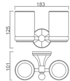
13402100 Double cups holder Material: Brass Finish: Chrome Number: 0026500
