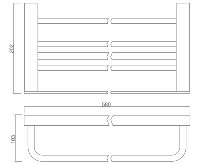
15901323 Towel rack Material: SUS304 Finish: Gun gray Number: 0083400
