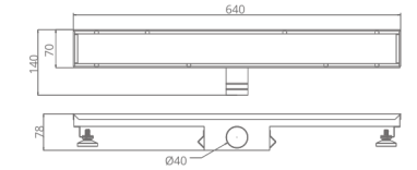
6521030 1 Floor drain Material: SUS304 Finish: Brushed Number: 0110800
