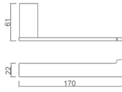
15801301 Tissue holder Material: SUS304 Finish: Brushed Number: 0020800
