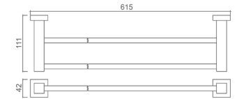
22102122 Double towel bar Material: Brass Finish: Black Number: 0049300
