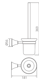
16601100 Toilet brush holder Material: Brass Finish: Chrome Number: 0019950
