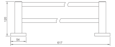
10102323 Double towel bar Material: SUS304 Finish: Gun gray Number: 0039000
