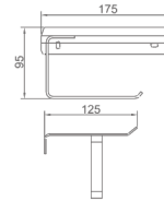
10812323 Tissue holder Material: SUS304 Finish: Gun gray Number: 0026000
