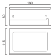
15803301 Tissue holder Material: SUS304 Finish: Brushed Number: 0024200
