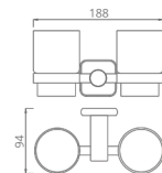
V1402322 Double cups holder Material: SUS304 Finish: Black Number: 0021500
