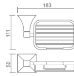
21502109 Soap basket Material: Brass Finish: Black Number: 0028750
