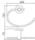
10201323 Towel ring Material: SUS304 Finish: Gun gray Number: 0023760
