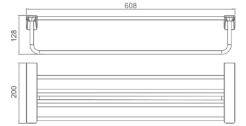
29901400 Towel rack Material: Zinc alloy Finish: Chrome Number: 0052500
