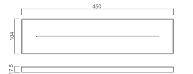
15701323 Shelf Material: Brass Finish: Gun gray Number: 0083460
