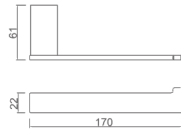
15801323 Tissue holder Material: SUS304 Finish: Gun gray Number: 0029900
