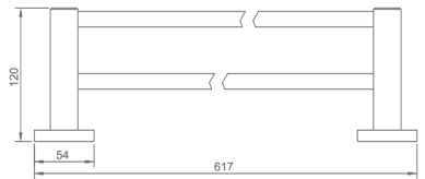
10102301 Double towel bar Material: SUS304 Finish: Brushed Number: 0020450
