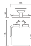
27802100 Tissue holder Material: Brass Finish: Chrome Number: 0022500
