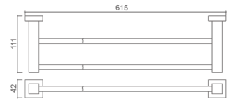
22102100 Double towel bar Material: Brass Finish: Chrome Number: 0041200
