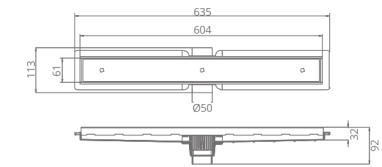
65220301 Floor drain Material: SUS304 Finish: Brushed Number: 0059800
