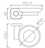
V1501322 Soap holder Material: SUS304 Finish: Black Number: 0017800
