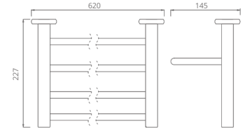
V1901322 Towel rack Material: SUS304 Finish: Black Number: 0049800
