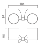
21402109 Double cups holder Material: Brass Finish: Black Number: 0030850
