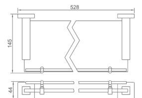
22711100 Glass shelf Material: Brass Finish: Chrome Number: 0039650
