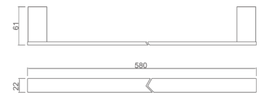
1510 13 0 1 Single towel bar Material: SUS304 Finish: Brushed Number: 0024850
