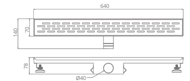
65230301 Floor drain Material: SUS304 Finish: Brushed Number: 0116800
