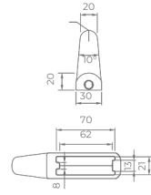
V3301302 Clothes hook Material: SUS304 Finish: Chrome Number: 0008600
