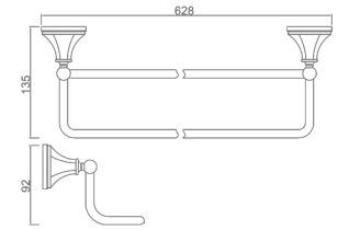
13102100 Double towel bar Material: Brass Finish: Chrome Number: 0041500
