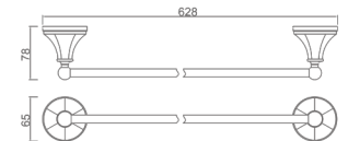
13101100 Single towel bar Material: Brass Finish: Chrome Number: 0032800
