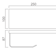
15802301 Tissue holder Material: SUS304 Finish: Brushed Number: 0038300
