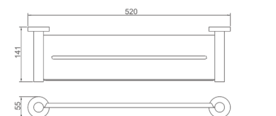
10701301 Single shelf Material: SUS304 Finish: Brushed Number: 0032500
