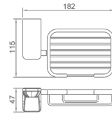
29502400 Soap basket Material: Zinc alloy Finish: Chrome Number: 0019000
