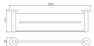
10701323 Single shelf Material: SUS304 Finish: Gun gray Number: 0046500
