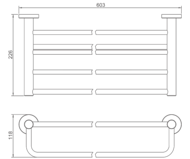
10901301 Towel rack Material: SUS304 Finish: Brushed Number: 0029800
