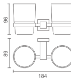
22402122 Double cups holder Material: Brass Finish: Black Number: 0027350
