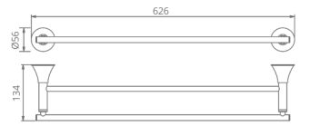
16102100 Single towel bar Material: Brass Finish: Chrome Number: 0036950
