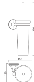
13601100 Toilet brush holder Material: Brass Finish: Chrome Number: 0032550
