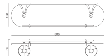
13701100 Glass shelf Material: Brass Finish: Chrome Number: 0045350
