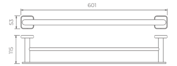
28102302 Double towel bar Material: SUS304 Finish: Chrome Number: 0033880
