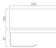
15802323 Tissue holder Material: SUS304 Finish: Gun gray Number: 0043920
