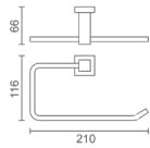
22201100 Towel ring Material: Brass Finish: Chrome Number: 0023350
