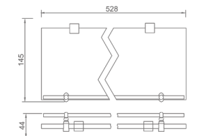
47503100 Glass shelf Material: Brass Finish: Chrome Number: 0019500
