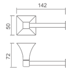
21801109 Tissue holder Material: Brass Finish: Black Number: 0022000
