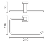
22201122 Towel ring Material: Brass Finish: Black Number: 0028050
