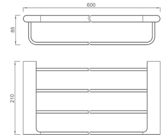
36901400 Towel rack Material: Zinc alloy Finish: Chrome Number: 0074520
