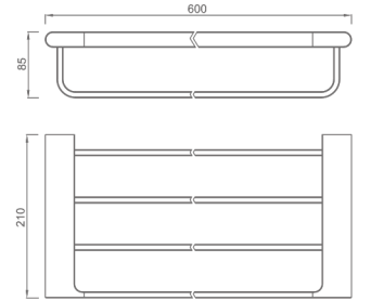
36901322 Towel rack Material: SUS304 Finish: Black Number: 0074550
