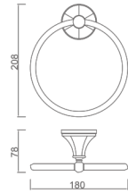
13201100 Towel ring Material: Brass Finish: Chrome Number: 0021250
