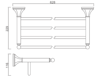
13901100 Towel rack Material: Brass Finish: Chrome Number: 0069800
