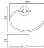
10201301 Towel ring Material: SUS304 Finish: Brushed Number: 0016000
