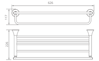
16902100 Towel rack Material: Brass Finish: Chrome Number: 0065800
