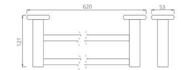
V1102322 Double towel bar Material: SUS304 Finish: Black Number: 0028900
