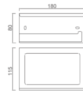
36812300 Tissue holder Material: Zinc alloy Finish: Chrome Number: 0025380
