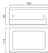
15803323 Tissue holder Material: SUS304 Finish: Gun gray Number: 0034850
